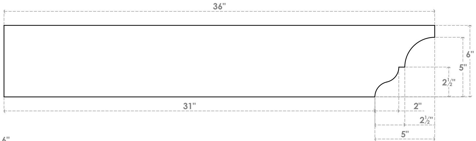
SIDE PROFILE
